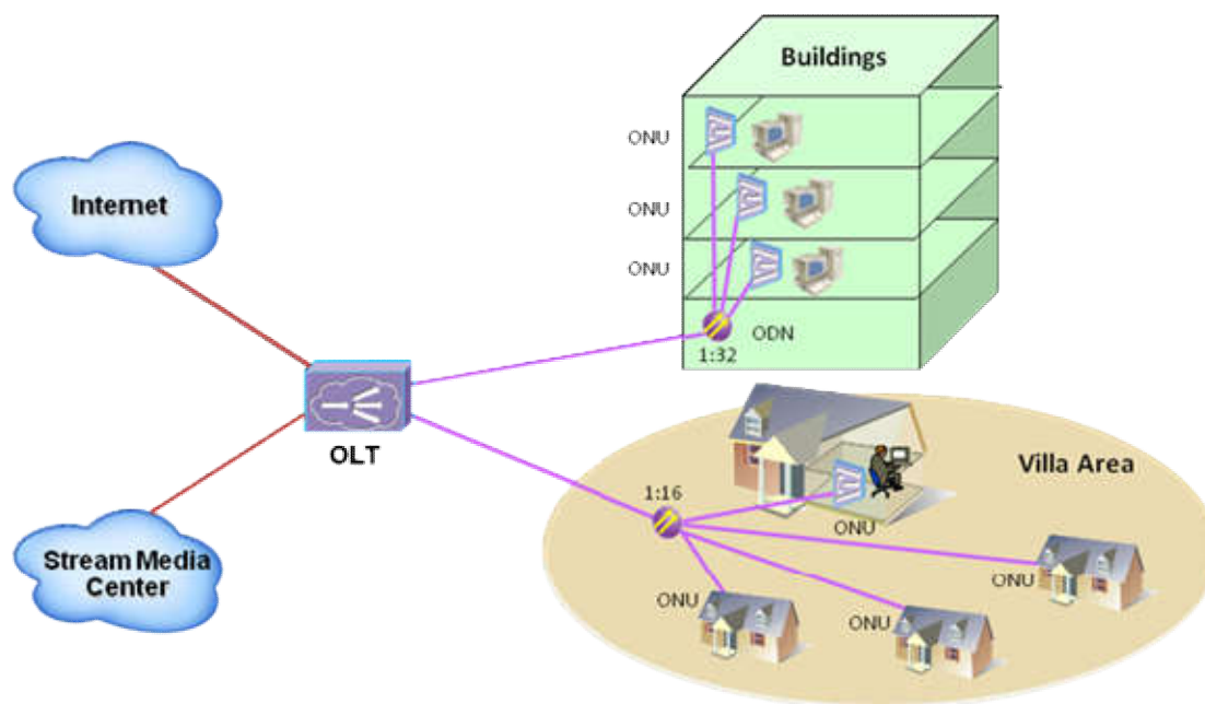
Picture 1-1RL801Gproducts Network diagram
